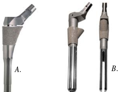
Figures 3A, and B. A: Apex Modular Stem. Note: Proximal modular shoulder/neck not fully seated (Courtesy George Cipolletti). B: S-Rom® Stem (Courtesy JISRF Archives).
